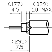
STRIPPING DIMENSION
